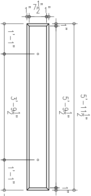
B PLAN
